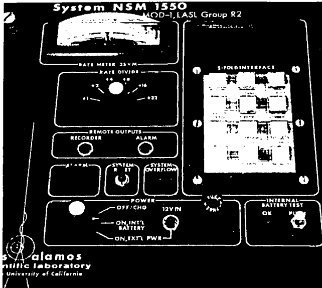
Fig. 5. The suitcase control panel.
